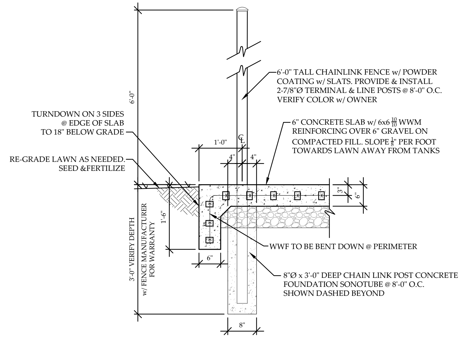
C FENCE POST DETAIL SCALE: 3/4"=1'-0"
