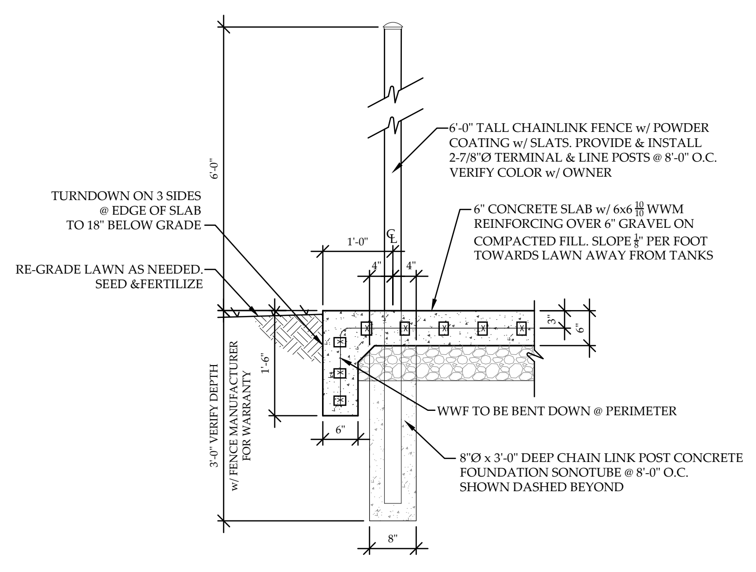
C FENCE POST DETAIL SCALE: 3/4"=1'-0"
